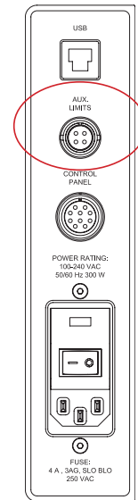
Fig. 2 ESM303 rear connectors
